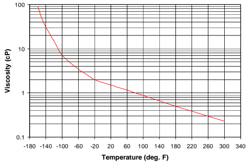
Viscosity of Dynalene MV®
