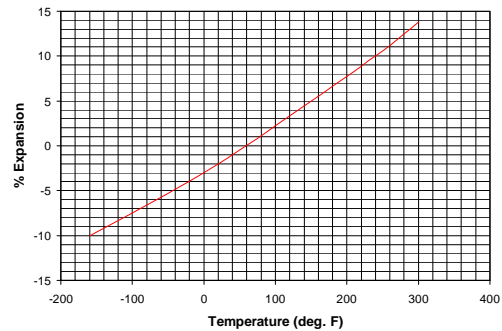
Volumetric Expansion of Dynalene MV®
